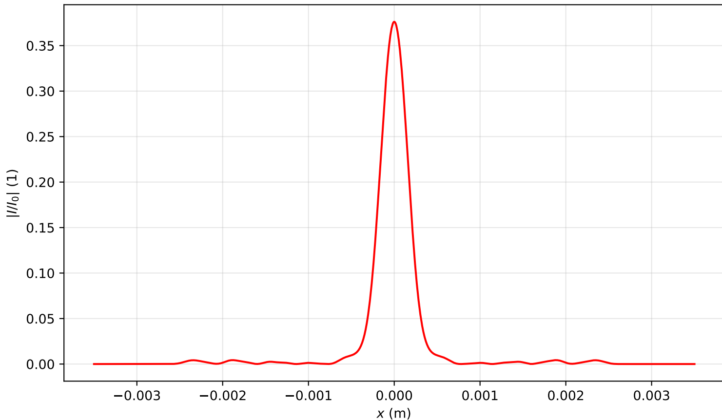
Intensity profile I(x, y = 0, z = 3.025)/I_0 , P_{in}=7.0P_{cr} , artificial time
